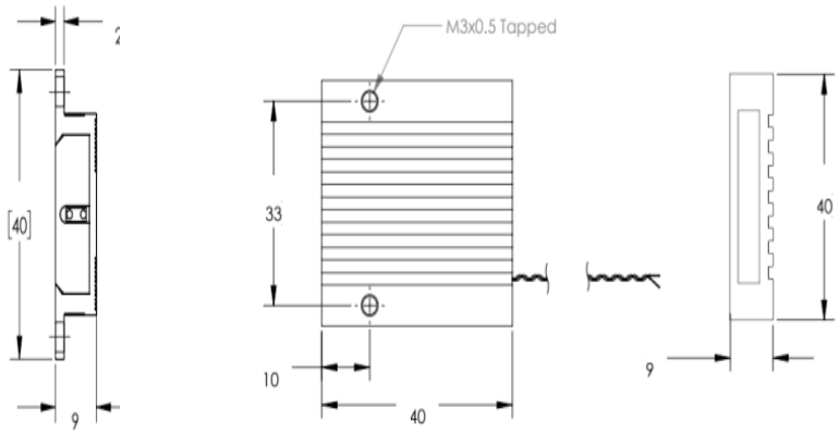
SPH 40*40 Model
