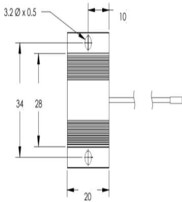
SPH 40*20 Model
